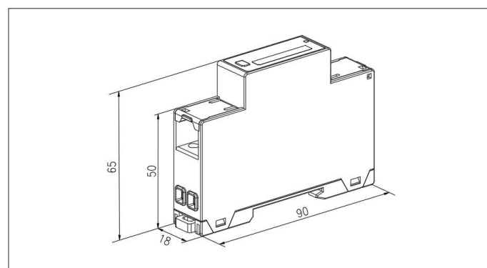
Meter-S
